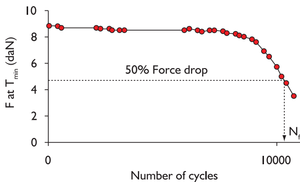
Figure 3. Thermal fatigue lifetime criterion.
