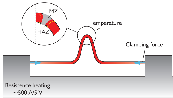
Figure 1. Thermal fatigue bench principle.
