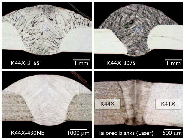
Figure 8. Initial microstructure of the weld seams – K44X MAG welding and Laser welding.
