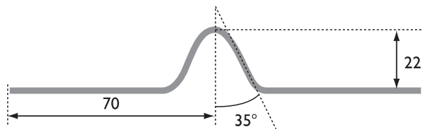
Figure 2. Sample geometry (thickness = 1.5 mm, width = 20 mm).
