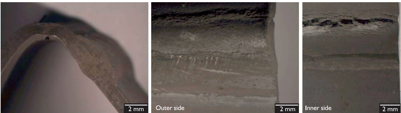
Figure 13. Binocular examination - K44X/430LNb.
