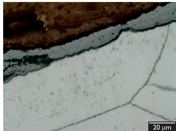
Figure 10. Post-mortem microstructural examination – K44X/430LNb.
