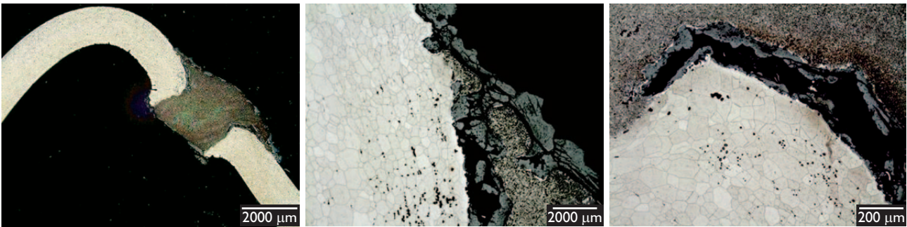
Figure 12. Post-mortem microstructural examination – K44X/316LSi.
