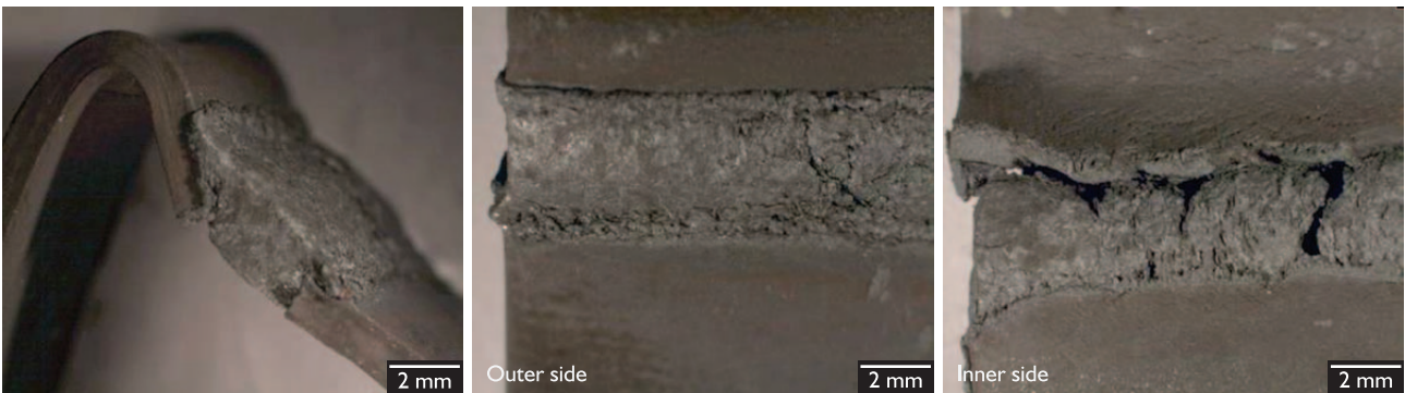
Figure 14. Binocular examination - K44X/307Si.
