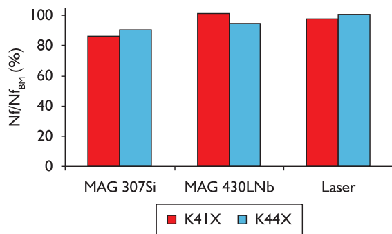
Figure 6. Weld seam lifetimes in comparison to base metal lifetime.
