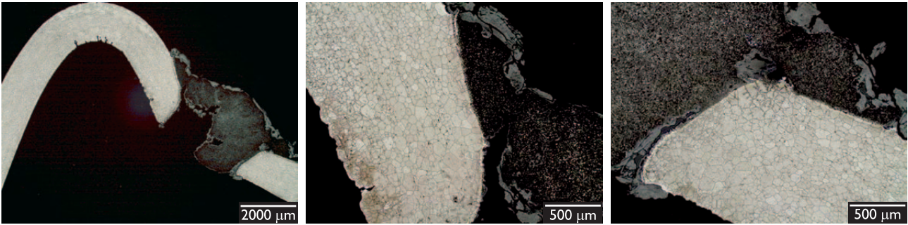
Figure 11. Post-mortem microstructural examination – K44X/307Si.
