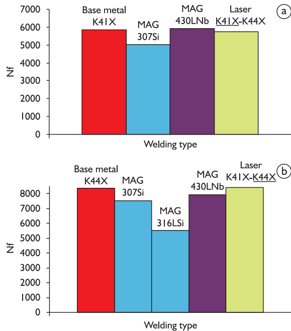
Figure 5. Mean thermal fatigue lifetimes of welded samples (3 samples per condition) for: a) K41X base metal; and b) K44X base metal.
