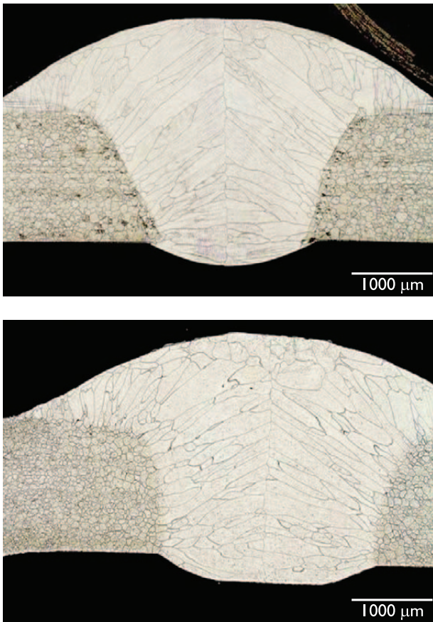
Figure 9. Microstructure of the K44X/430Nb before and after thermal fatigue test.
